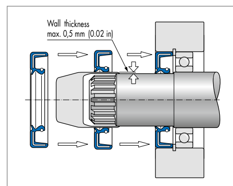
Fig. 13 Installation over a shaft with a keyway (also for a sharp-edged shoulder on shaft)
